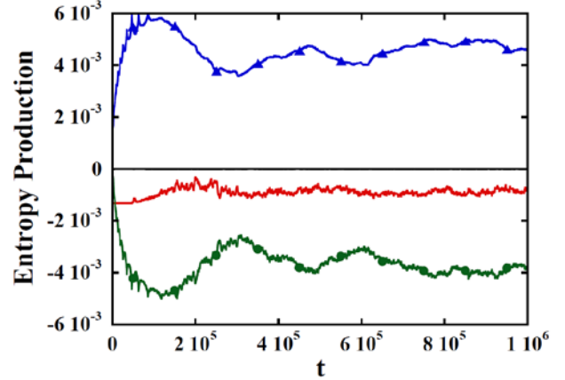
Fig. 2: Time evolution of entropy production related to macroscopic (red), microscopic (green) quantities and external heat input/output (blue). Black line shows the sum of them as a reference.
