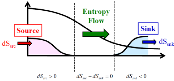
Fig. 1: Schematic picture of entropy dynamics in open system. Heat input at the core increases entropy whereas the output at the edge decreases entropy.
