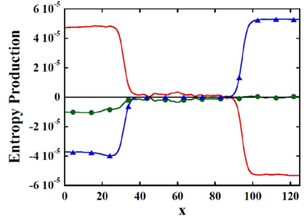
Fig. 3: Spatial profiles of entropy production. Each color line corresponds to same one in Fig. 2.
